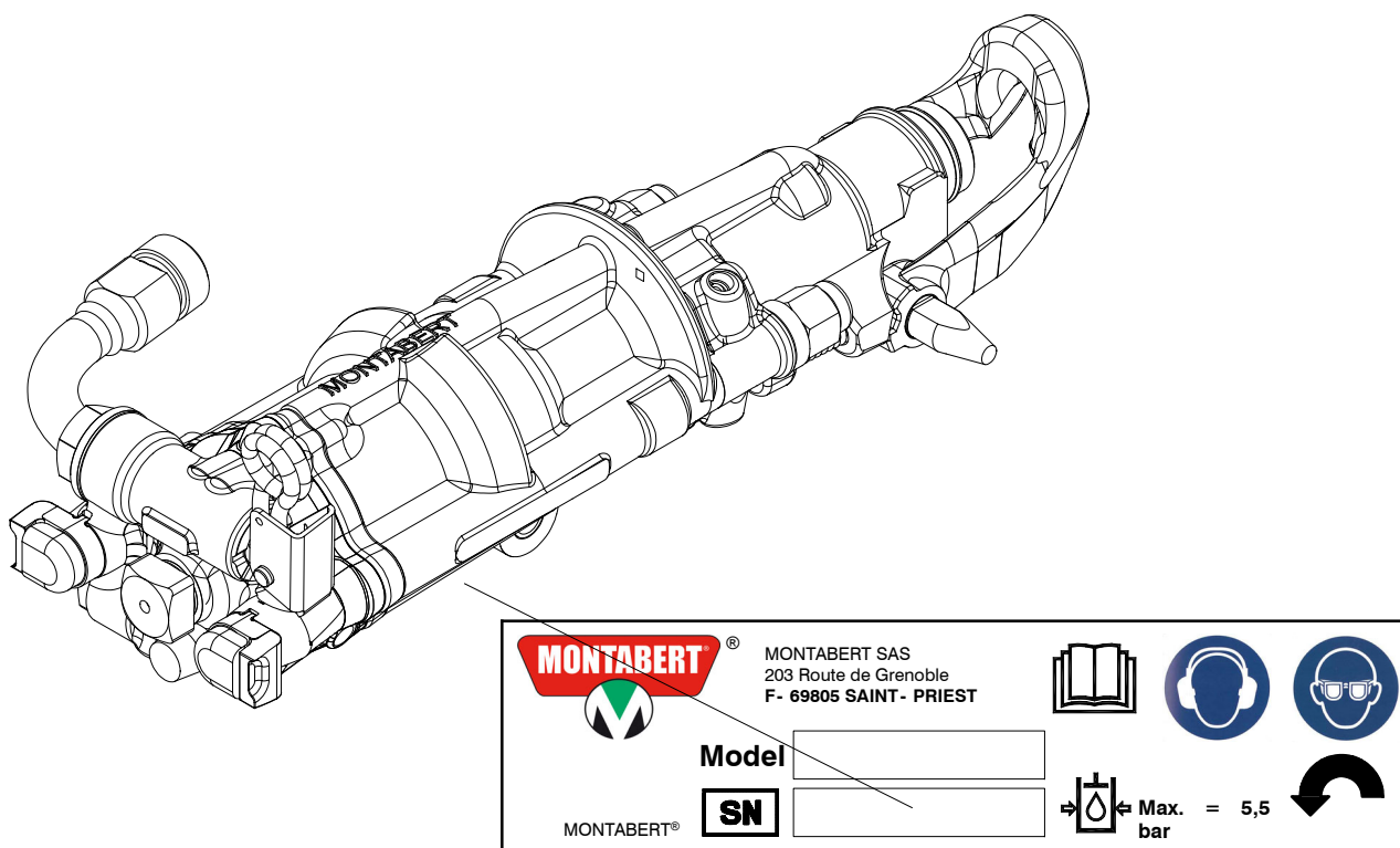
Identification plate
